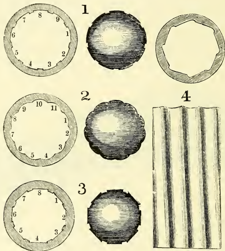
Grooving of Sporting Rifles.
